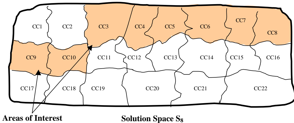
Figure 3.4 Example Solution Space With Conjugacy Class Partitions
