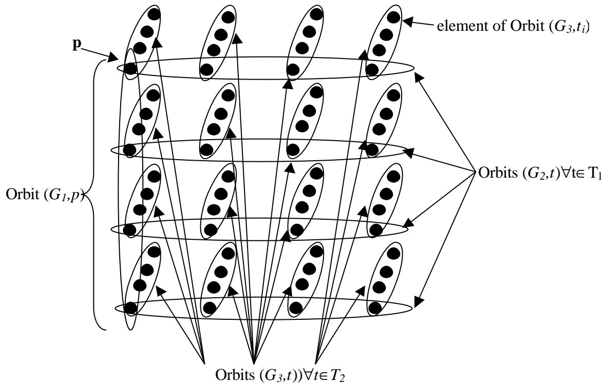
Figure 3.7 Orbital Plane Partitioning Through Successive Group Actions
