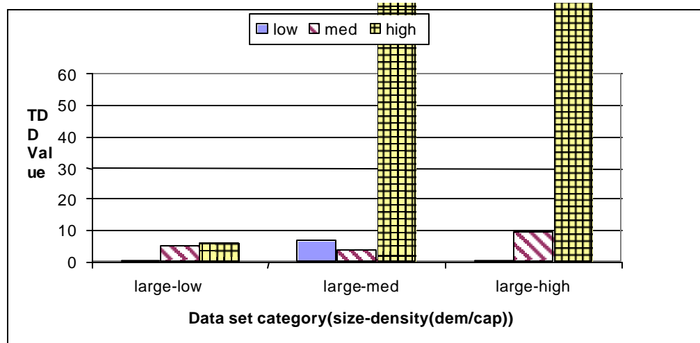
Figure 8.6 TDD Value Relative to Problem Density (Large Problems)
